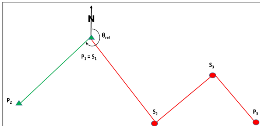
Fig. 2. Planimetric surveying supported on two reference points
